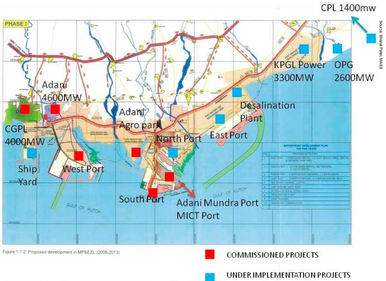
Figure 6.12: Proposed development in MPSEZL
