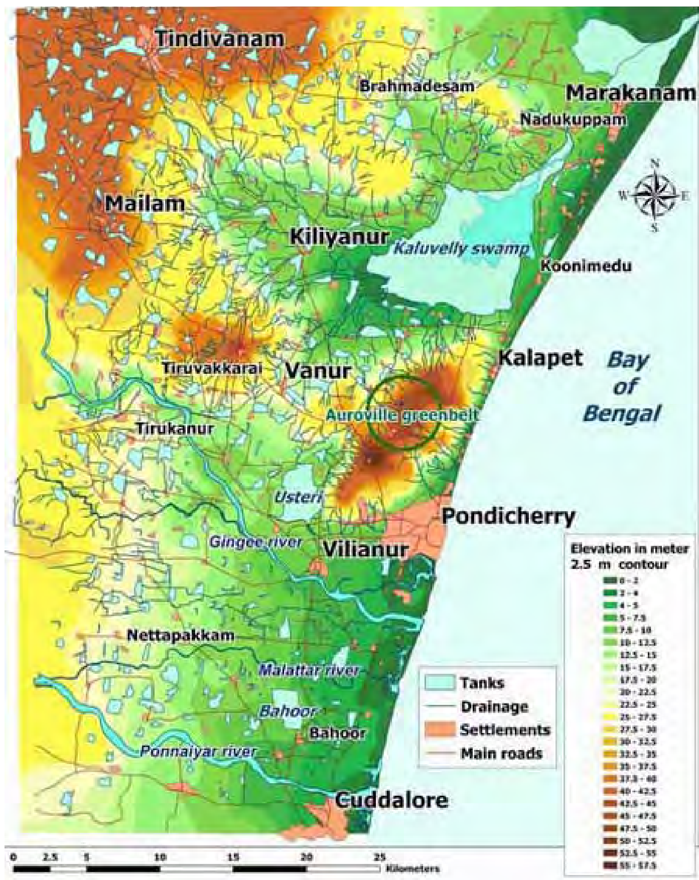
Elevation and hydrography of the PVAC region
